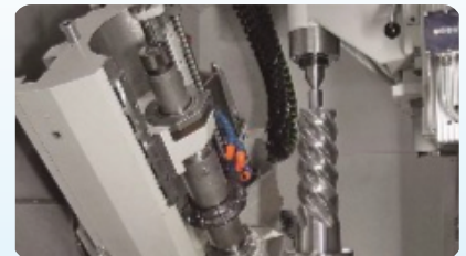
MODUL GEAR HOBBING MACHINES H600 - H800
